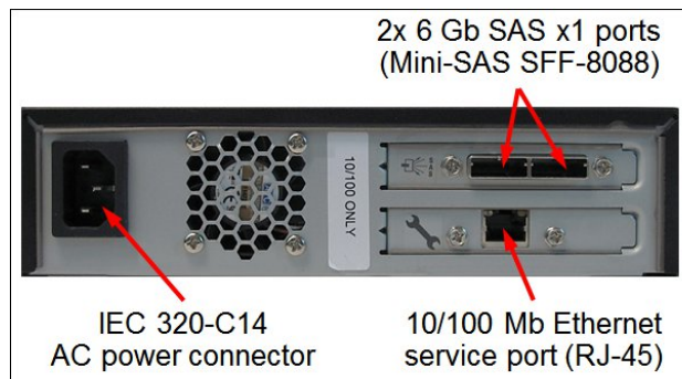
Figure 6. Rear view of the TS2280, or TS2270, or TS2260
